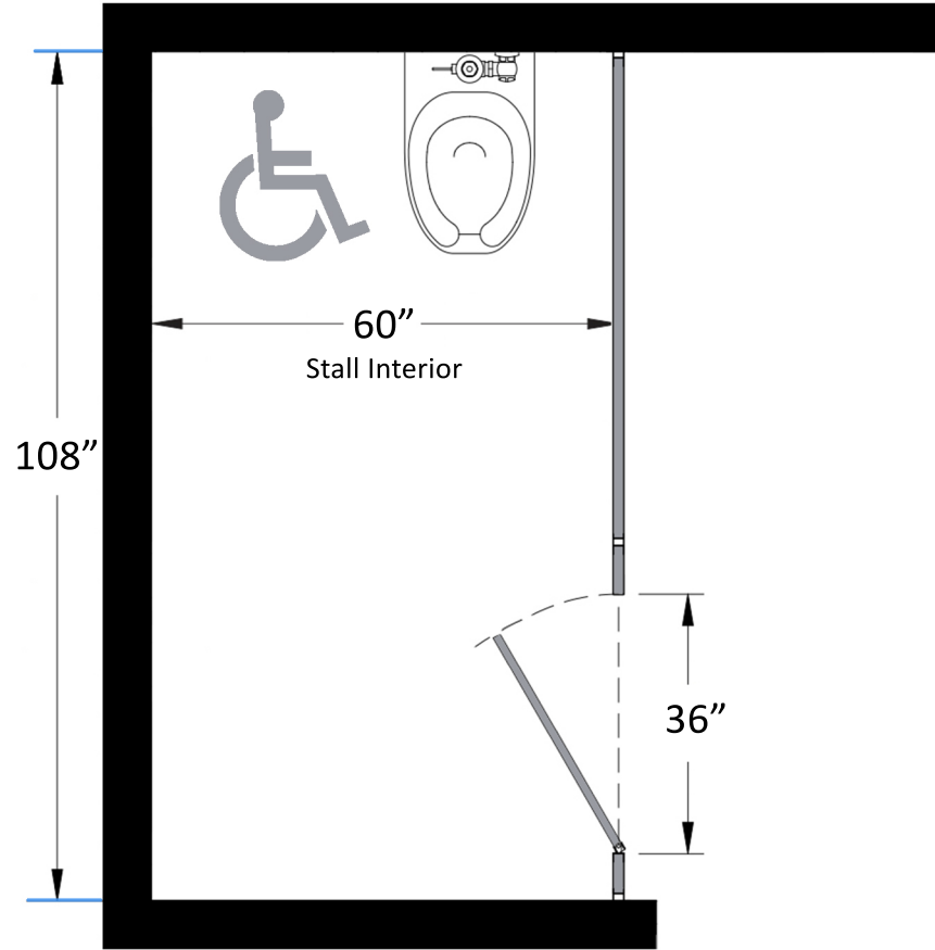
Bathroom Partitions - 1 Stall Alcove Left Hand ADA SKU: ALIC1LADA Standard Dimensions
